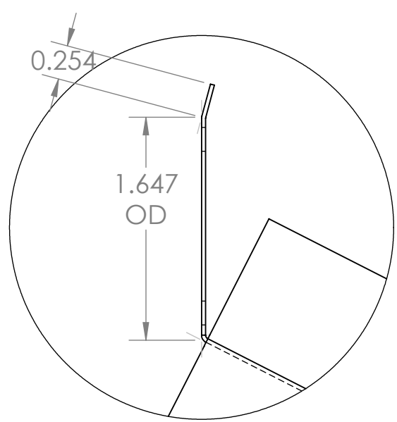
DETAIL E SCALE 1 : 1
